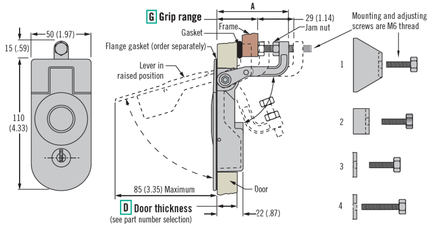
Brackets to Suit Door Thickness
